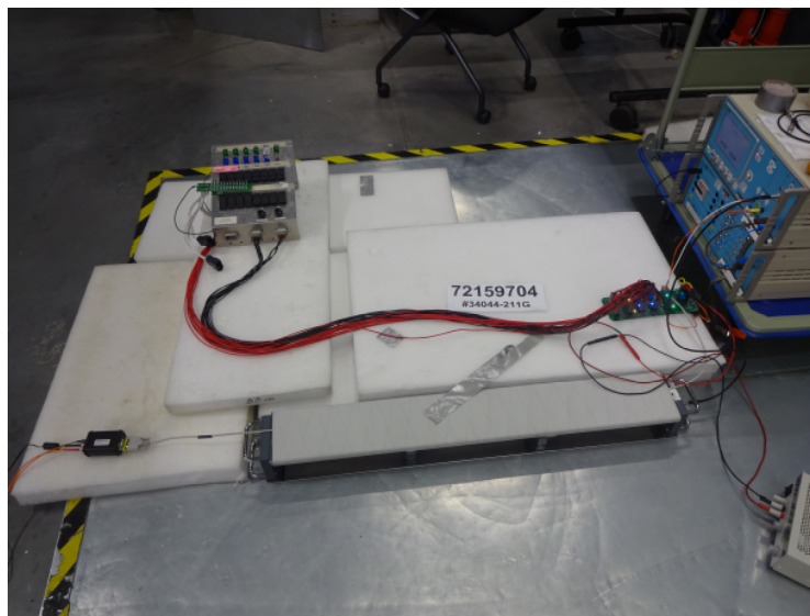
Photo setup (Communication Cable)
